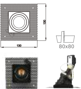
TS1 Fixed Mounting Ring IP Rating: IP20 Casting Color : White / Black / Customized Cut out 80x80mm
