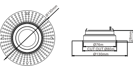
TR1 Fixed Mounting Ring IP Rating: IP20 Casting Color : White / Black / Customized Cut out Ø80mm
