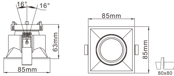
SQ16 Adjustable Mounting Ring Adjustable Angle 16° Casting Color : White / Black / Customized Cut out 80x80mm
