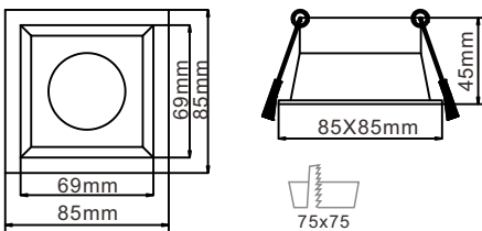
SQ17 Fixed Mounting Ring IP Rating: IP20 Casting Color : White / Black / Customized Cut out 75X75mm
