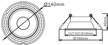
TRF5-W Fixed Mounting Ring IP Rating: IP20/IP44 Casting Color : White / Black / Customized Cut out Ø100mm
