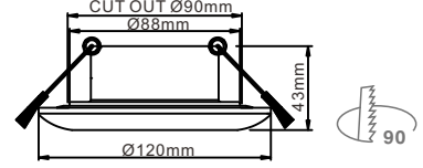
RF23 Fixed Mounting Ring IP Rating: IP20 / IP44 / IP65 Casting Color : White / Black / Customized Cut out Ø90mm
