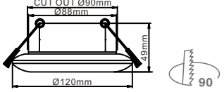
RF22 Fixed Mounting Ring IP Rating: IP20 / IP44 / IP65 Casting Color : White / Black / Customized Cut out Ø90mm
