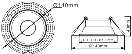
TRF6 Fixed Mounting Ring IP Rating: IP20/IP44 Casting Color : White / Black / Customized Cut out Ø100mm
