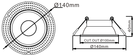
TRF15-W Fixed Mounting Ring IP Rating: IP20 / IP44 Casting Color : White / Black / Customized Cut out Ø100mm
