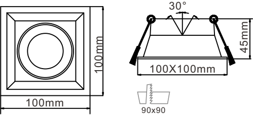
SQ18 Adjustable Mounting Ring Adjustable Angle 30° Casting Color : White / Black / Customized Cut out 90x90mm
