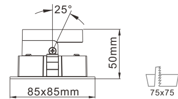
SQ15 Adjustable Mounting Ring Adjustable Angle 25° Casting Color : White / Black / Customized Cut out 75x75mm
