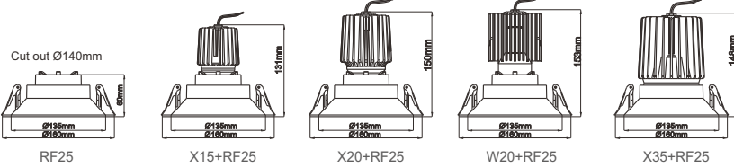
RF25 Fixed Mounting Ring IP Rating: IP20/IP44/IP65 Casting Color : White / Black / Customized Cut out Ø140mm
