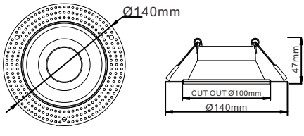
TRF2 Fixed Mounting Ring IP Rating: IP20 / IP44 / IP65 Casting Color : White / Black / Customized Cut out Ø100mm
