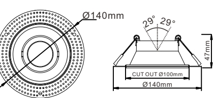
TRA2 Adjustable Mounting Ring Adjustable Angle 29° Casting Color : White / Black / Customized Cut out Ø100mm
